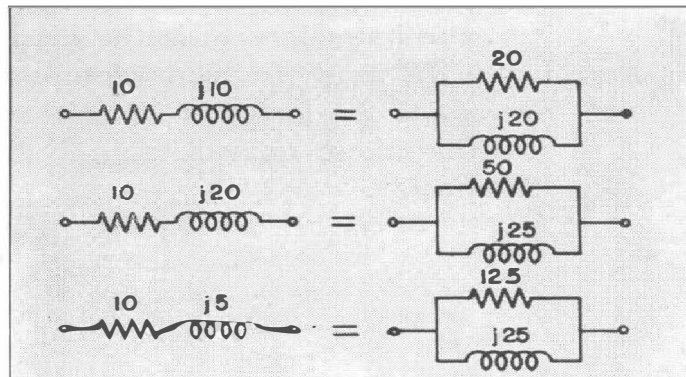
FIGURE 1. Examples of equivalent series and parallel circuits.
