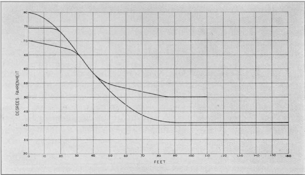
Temperature of water as a function of depth. Near the surface, the temperature depends upon the time of day and the weather for the preceding several hours, and the three branches of the curve illustrate the differences encountered. At depths below about 40 feet the curve has two branches, one for ultimate depths of about 100 feet, the other for ultimate depths of 160 feet or more.
