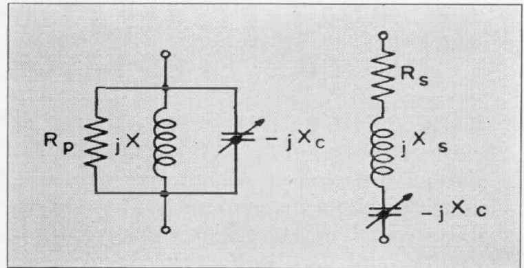
FIGURE 2. Series and parallel resonant circuits. The capacitance necessary to resonate with a given inductance will depend upon whether the elements are connected in series or in parallel.
